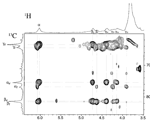
Figure 2. Aliphatic region of a 2D HMQC-TOCSY experiment showing syringyl \beta -ether units and the excellent dispersion of erythro - and threo -isomers. NMR conditions: Bruker AMX-360, 5 mm tube, 5 mm normal mode probe (proton coil outermost), Bruker pulse program "invbmltp" [phase-sensitive, inverse-detected C-H correlation using a BIRD sequence for minimizing protons bound to ^{12}\text{C} -carbons (300 ms inversion-recovery delay), and MLEV-17 Hartman-Hahn mixing (100 ms)], spectral widths 4000 Hz ( ^1\text{H} ) and 13 100 Hz ( ^{13}\text{C} ), acquisition time 0.26 s, relaxation delay 1 s, 256 increments of 520-scan 2K FIDs, total acquisition time 62 h. Processing: cosine-bell apodization in both dimensions, phase-sensitive (TPPI) Fourier transform with zero-filling to 1K by 1K real data points resulting in 3.9 ( ^1\text{H} ) and 12.8 ( ^{13}\text{C} ) Hz/pt resolutions.
