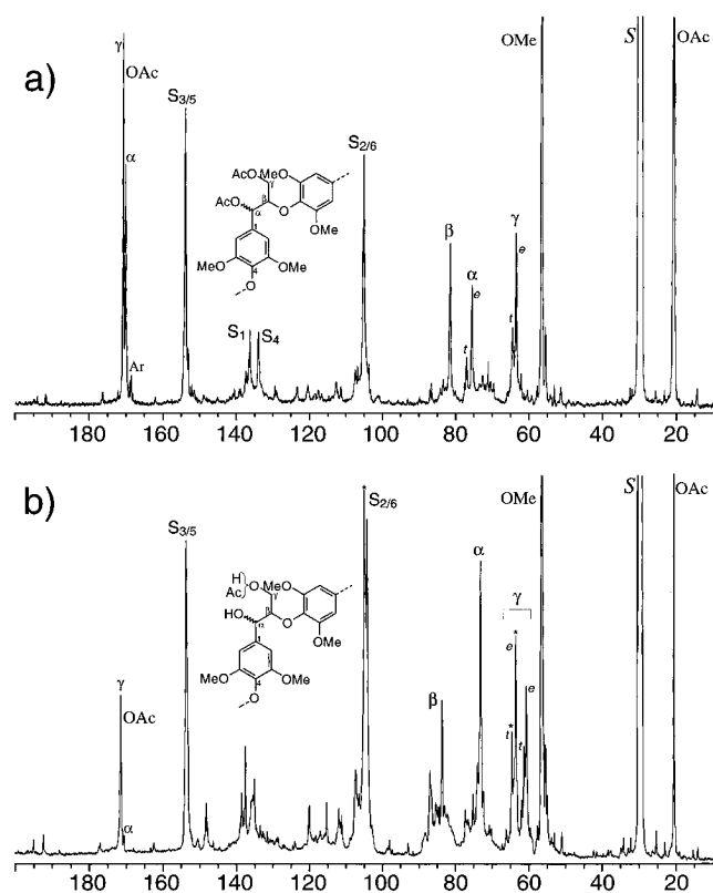
Figure 1. ^{13}\text{C} NMR spectra of the isolated kenaf lignins showing the preponderance of syringyl peaks. Assignments are for \beta -ethers: (a) acetylated, (b) underivatized. * indicates easily identifiable peaks that result from acetate substitution. NMR conditions (qualitative): Bruker AMX-360, 10 mm tube/probe, temperature 300 K, 70^\circ pulse width, acquisition time 0.7 s, relaxation delay 0.3 s (total recycle delay, 1 s), ca. 50 000 scans, Waltz-16 decoupling: (a) 373 mg in 2.4 mL of acetone- d_6 , (b) 330 mg in 2.4 mL of 9:1 acetone- d_6 : \text{D}_2\text{O} .
